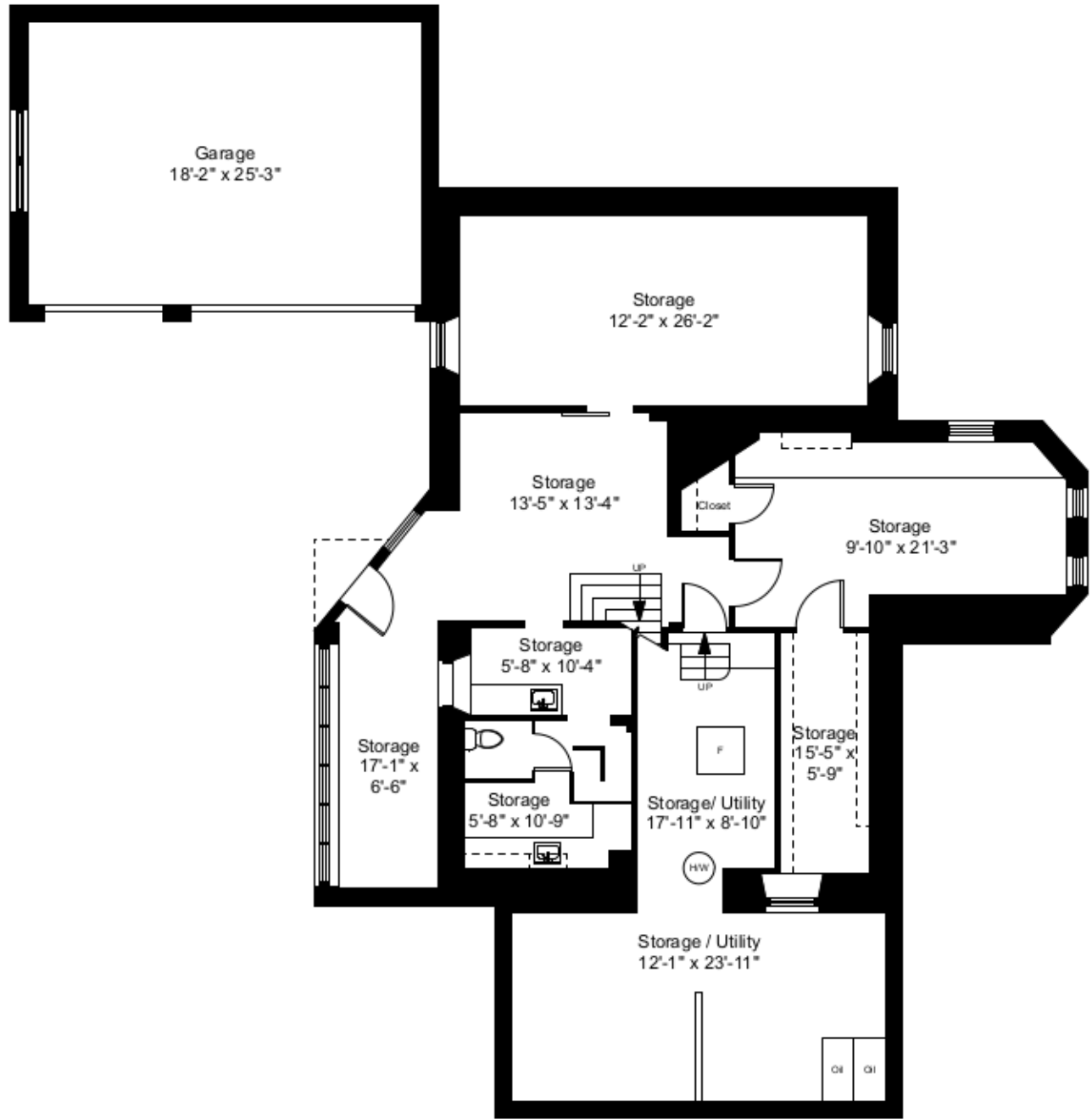
Basement Plan Ceiling Height = 8'-10"
