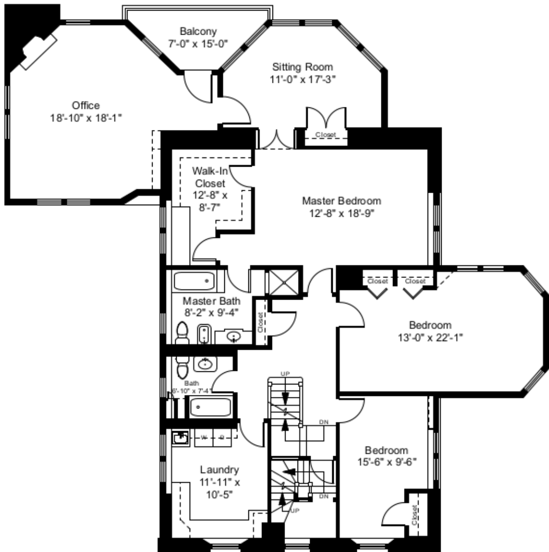
Second Floor Plan Ceiling Height = 8'-9"
